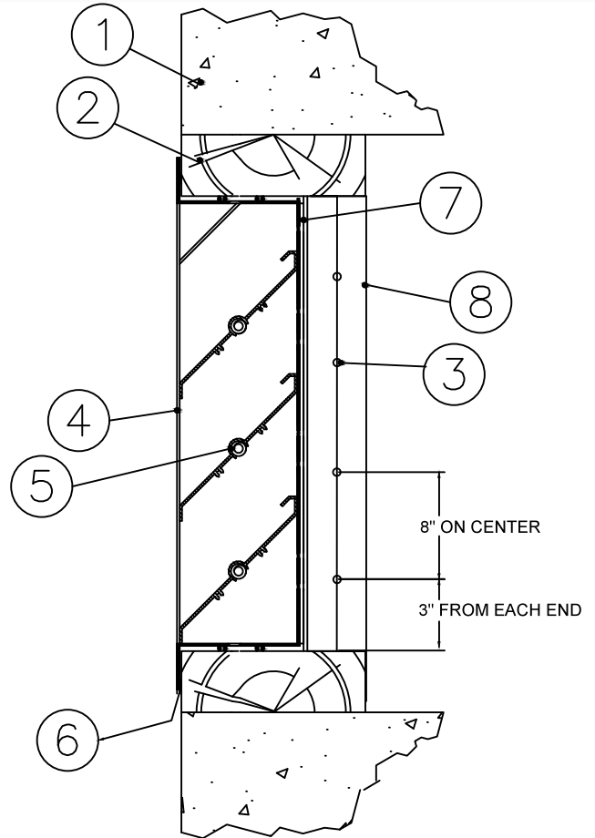
INSTALLING TO WOODEN FRAME
